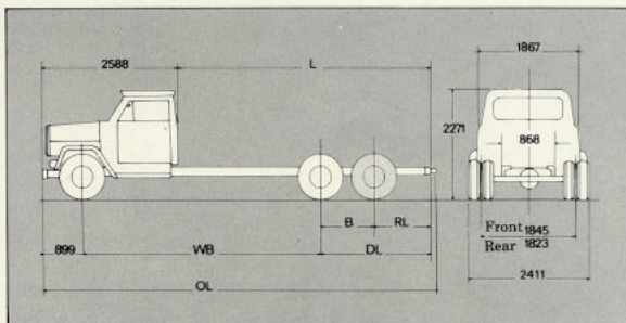
DIMENSIONS (mm)
